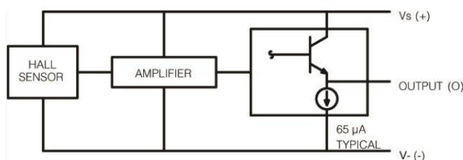
Figure 1. Current Sourcing Output Block Diagram
