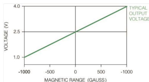
Figure 2. Transfer Characteristics ( V_S = 5.0\text{ Vdc} )
